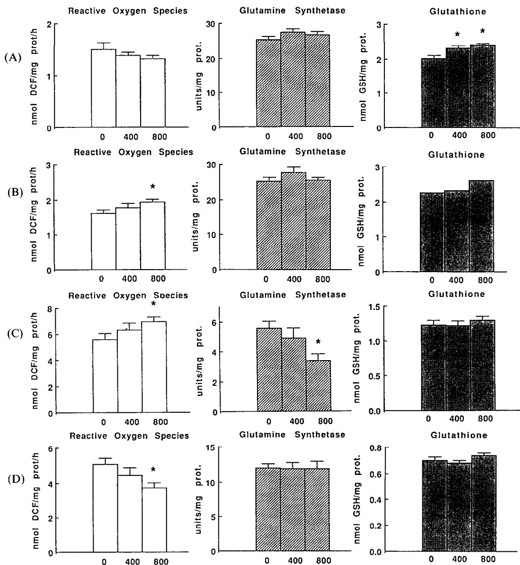
Fig. 1. Effects of 3 weeks inhalation exposure 6 hr/day, 7 days/week to 0, 400 or 800 ppm of dearomatized white spirit on the rates of generation of ROS, glutamine synthetase activities and levels of GSH in P2 fraction of hemispheres (A), hippocampus (B), liver (C) and left kidney (D). Values are the means \pm SEM from 10 animals. * = value differs significantly from the control level ( P < 0.05 , two-tailed test).
